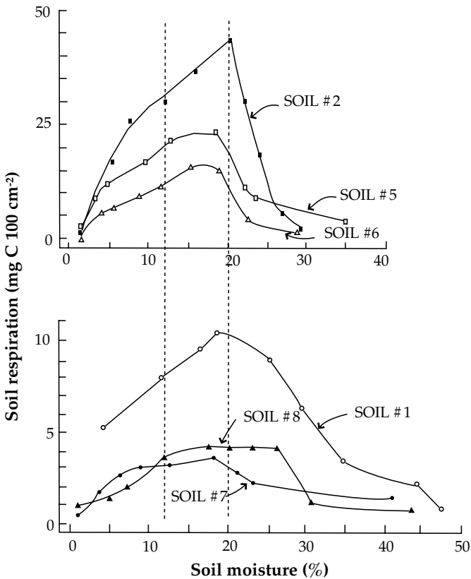
Figure 8. Relationship between soil respiration and soil moisture. Source: Boyd and Pipoppinyo (1994).
