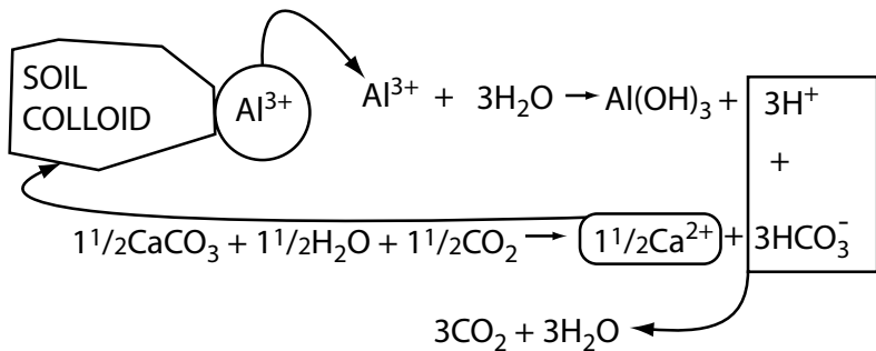
Figure 6. Model for neutralization of exchangeable acidity in soil by calcium carbonate.
